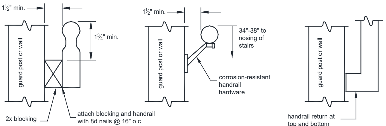
FIGURE 44: HANDRAILS
