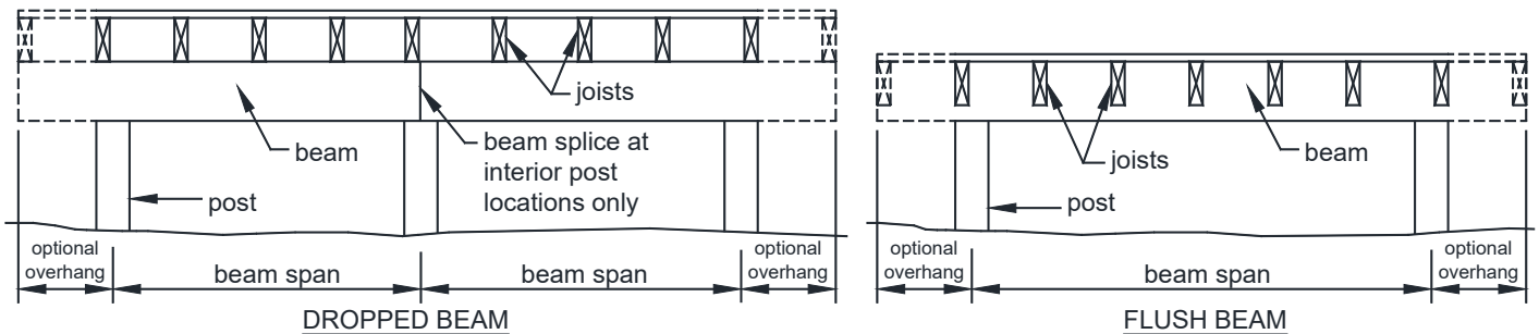
FIGURE 13: BEAM TYPES
