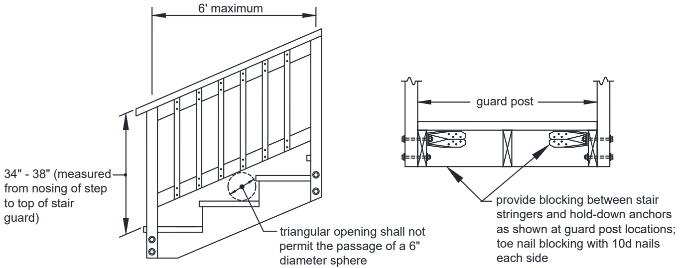
FIGURE 43: STAIR GUARD
