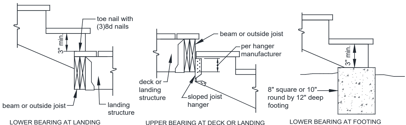
FIGURE 40: STRINGER BEARING
