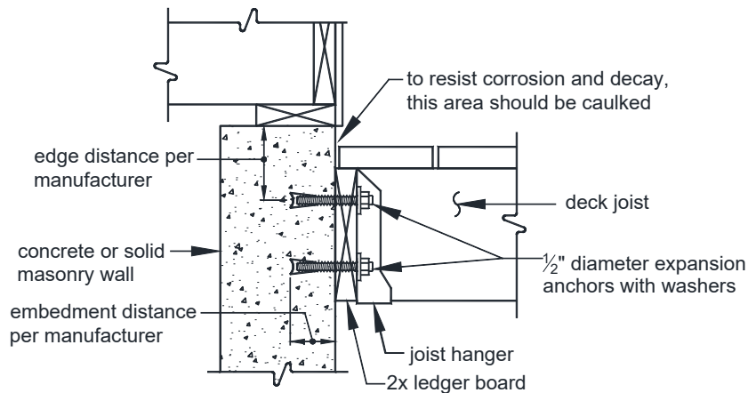
FIGURE 23: LEDGER BOARD-TO-SOLID FOUNDATION ATTACHMENT
