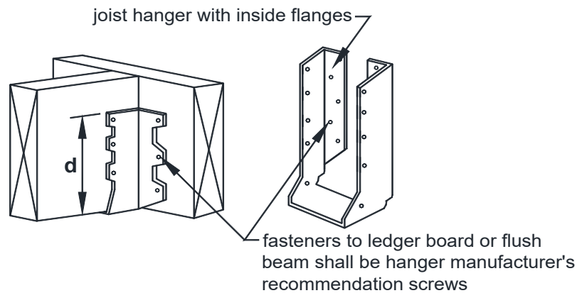
FIGURE 11: JOIST HANGERS
