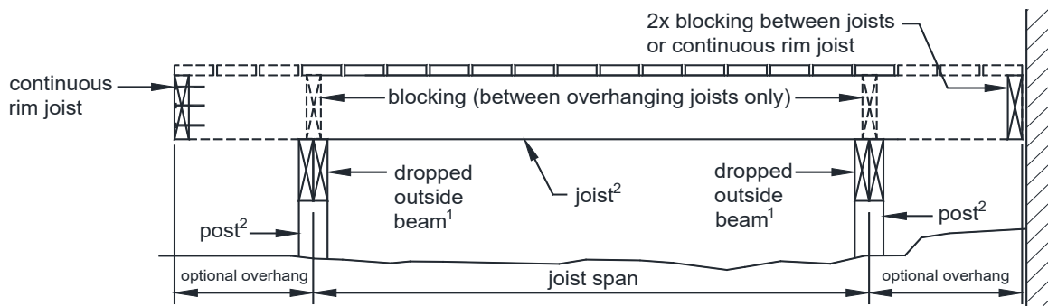
FIGURE 9: JOISTS WITH FREESTANDING DECKS
