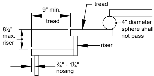
FIGURE 39: TREADS AND RISERS
