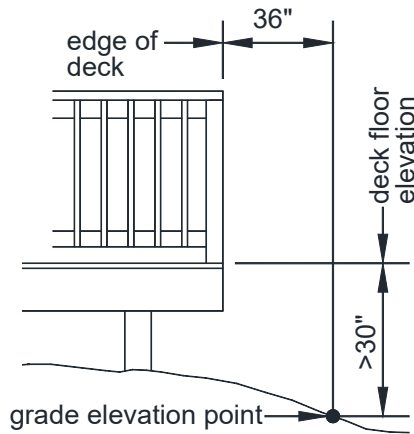
FIGURE 34: WHEN A GUARD IS REQUIRED
