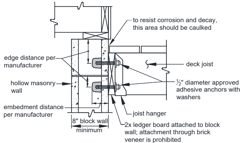
FIGURE 24: LEDGER BOARD-TO-HOLLOW FOUNDATION ATTACHMENT
