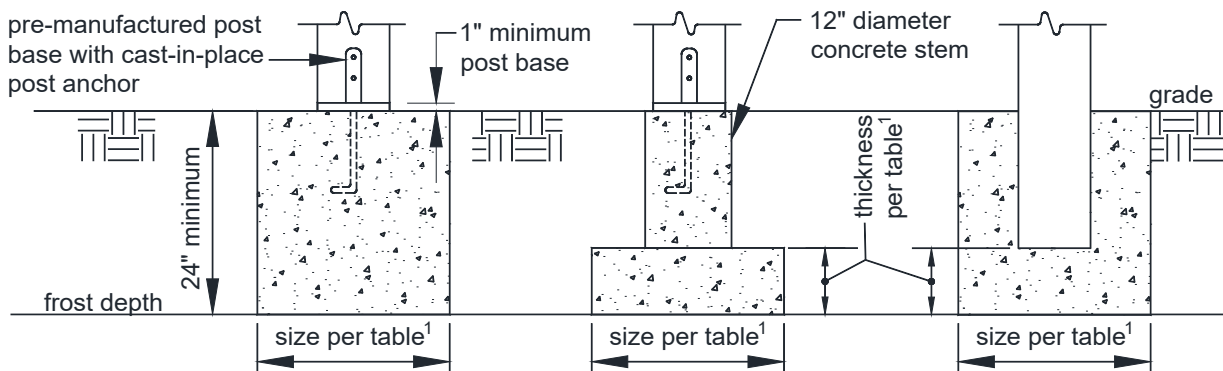
FIGURE 17: FOOTINGS
