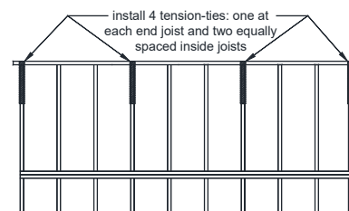
FIGURE 28: METHOD 1 - TENSION TIE LOCATIONS
