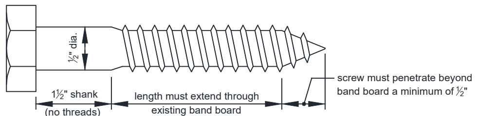
FIGURE 27: LAG SCREW
