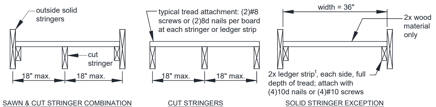
FIGURE 42: STRINGER TREADS
