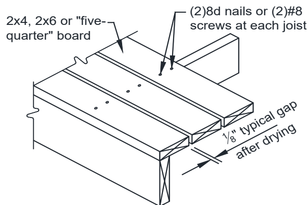
FIGURE 1: TYPICAL DECKING
