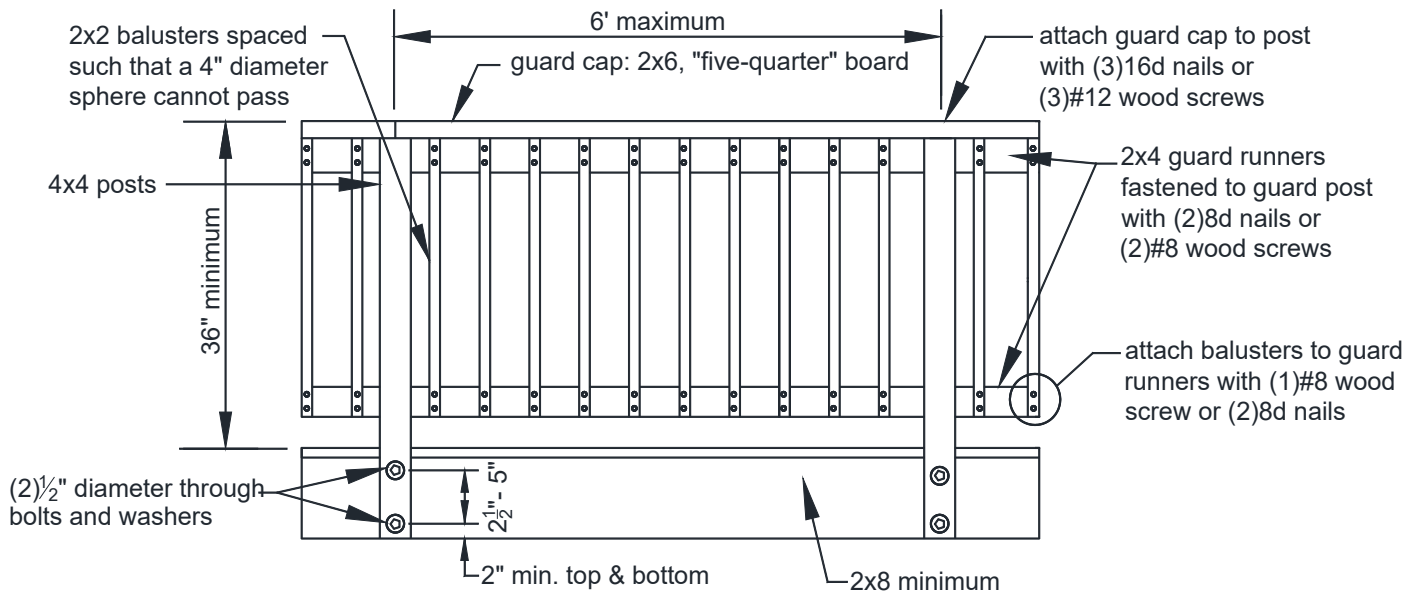
FIGURE 35: GUARD CONSTRUCTION
