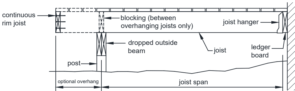
FIGURE 5: SINGLE SPAN DECK - JOISTS ATTACHED AT HOUSE WITH DROPPED BEAM
