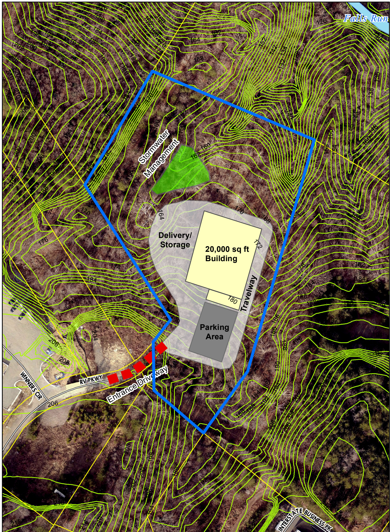
TAX MAP PARCEL NO. 45-98 POTENTIAL DEVELOPMENT SCENARIO
