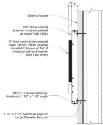
Section @ Non-Illuminated Letters
